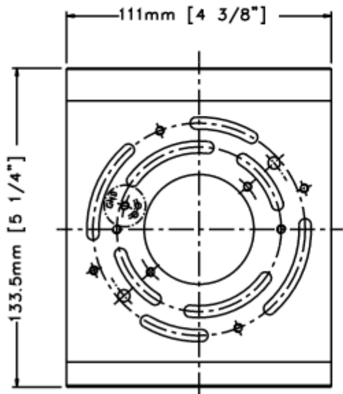
MOUNTING PLATE
