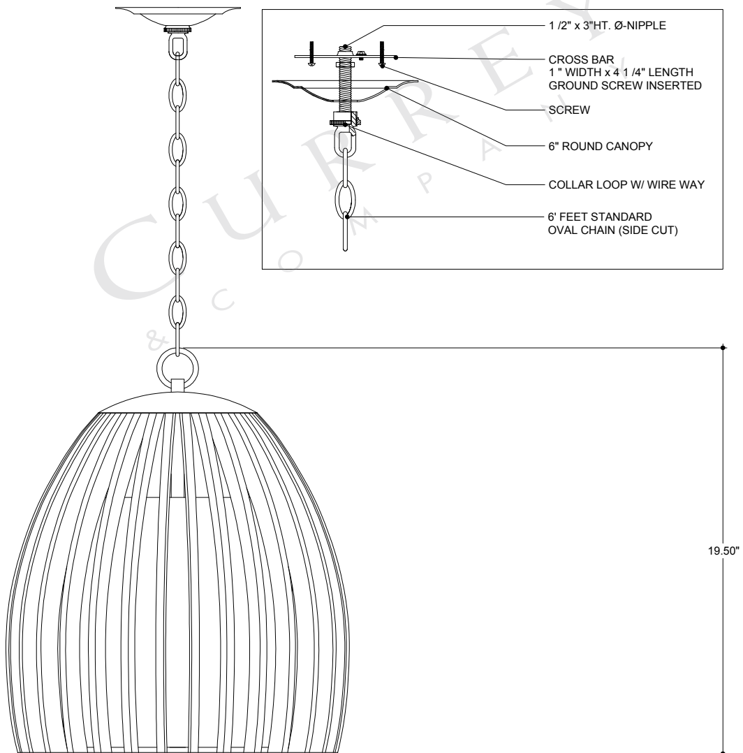
FRONT VIEW
