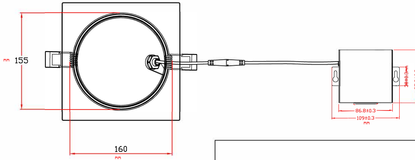
6" LED SQUARE GIMBAL SLIM LIGHT
