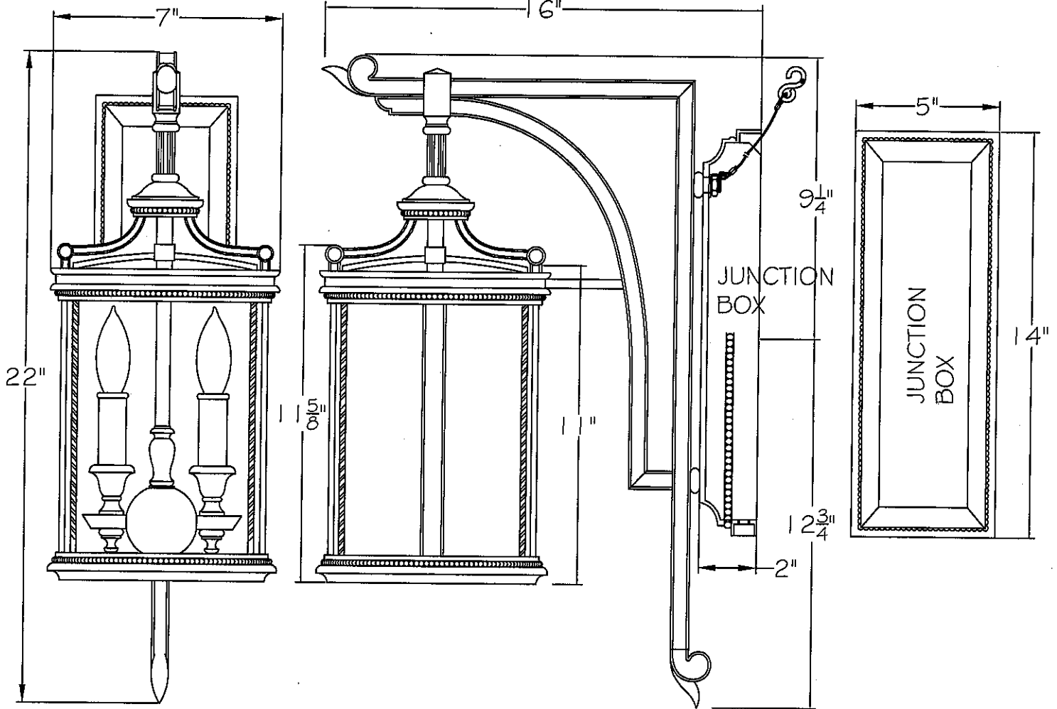
SIDE VIEW
