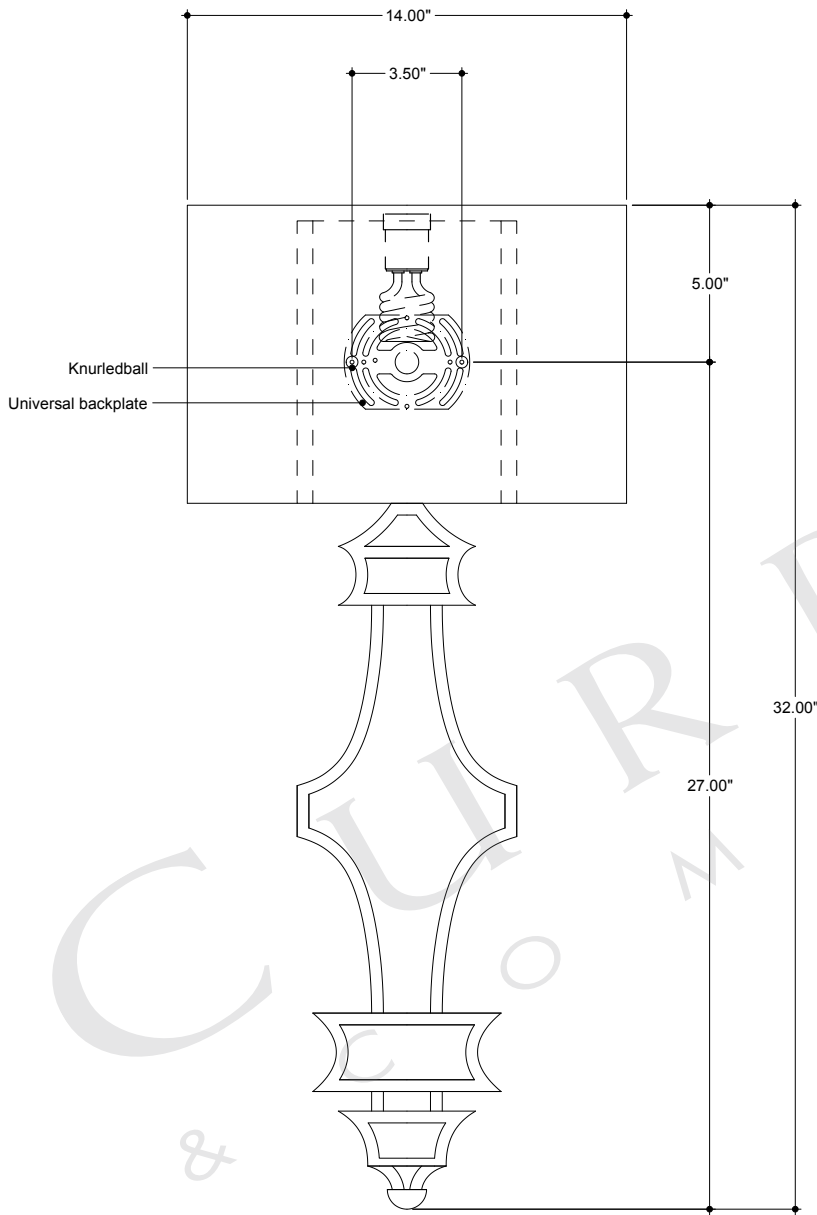
FRONT VIEW
