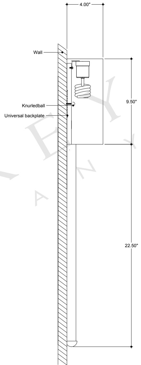
SIDE VIEW
